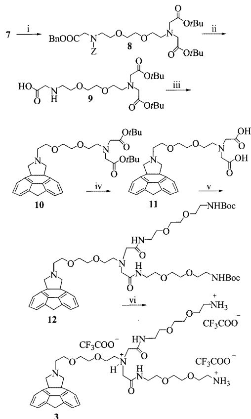
Scheme 2. i: K 2 CO 3 , tert -butyl bromoacetate, THF; ii: H 2 , Pd/C, methanol; iii: C 60 , paraformaldehyde, toluene, Δ; iv: TFA, CH 2 Cl 2 ; v: EDC·HCl, HOBt, 4 , dioxane; vi: TFA, CH 2 Cl 2
