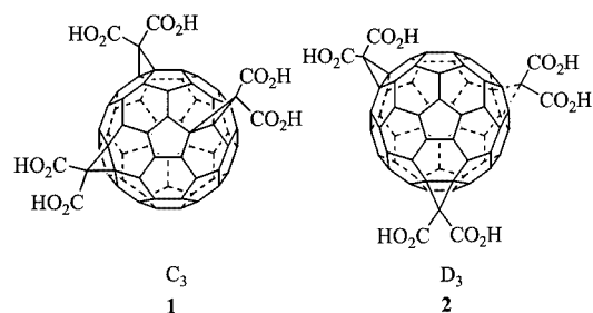
Figure 1. Isomeric C 60 -tris(malonic acid) derivatives 1 (C 3 ) and 2 (D 3 )
