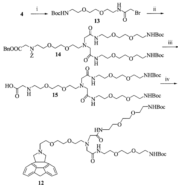
Scheme 3. i: Bromoacetyl bromide, TEA, \text{CH}_2\text{Cl}_2 ; ii: 7 , TEA, \text{CH}_2\text{Cl}_2 ; iii: \text{H}_2 , Pd/C, methanol; iv: \text{C}_{60} , paraformaldehyde, toluene, \Delta
